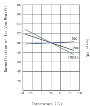
Temperature Curves of Isc, Voc, Pmax under Different Temperatures
