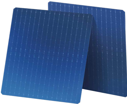
TC-NG12R16B 182.2mm×210mm±0.5mm φ272mm±0.5mm
