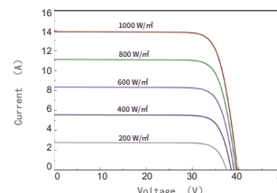
Current and voltage curves under different irradiances
